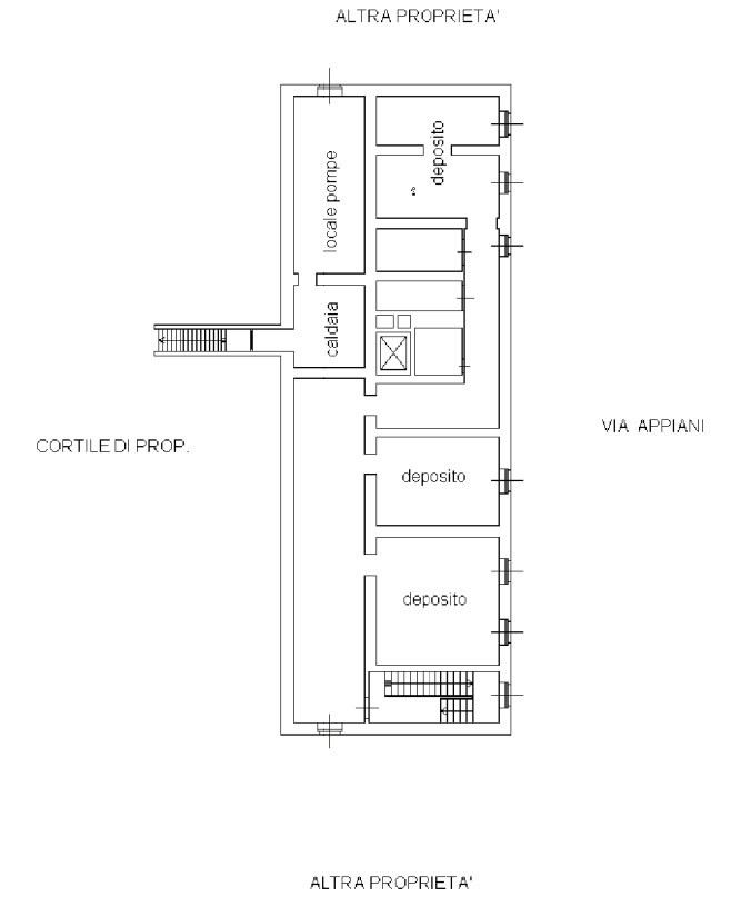
PIANO INTERRATO H=m. 2,80
